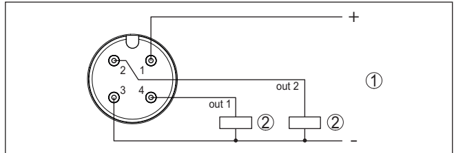
Fig. 7: Wiring plan M12 x 1 plug - Transistor output, three-wire
