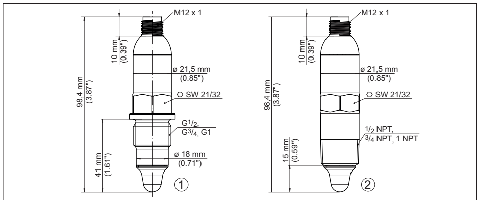
Fig. 9: VEGAPOINT 11, standard version - thread
