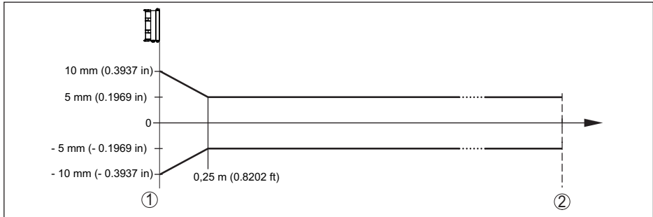
Fig. 17: Deviation under reference conditions
