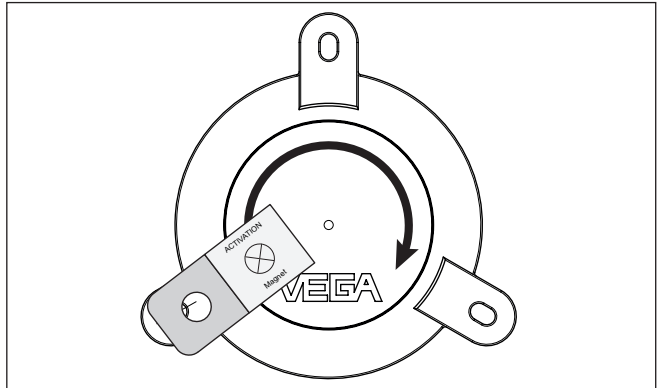
Fig. 9: Activate sensor - Magnet
