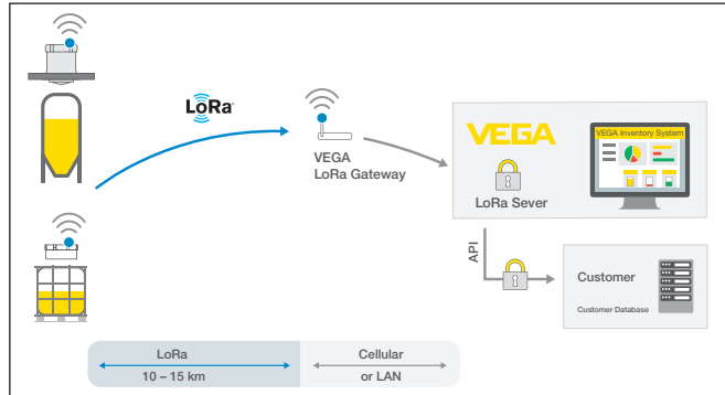
Fig. 11: Wireless measured value transmission via LoRa-WAN, LoRa server to the VEGA Inventory System
