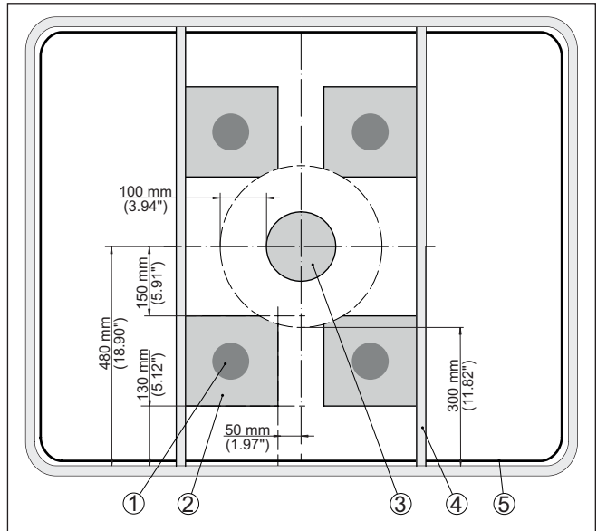
Fig. 5: Mounting position on the tank ceiling
