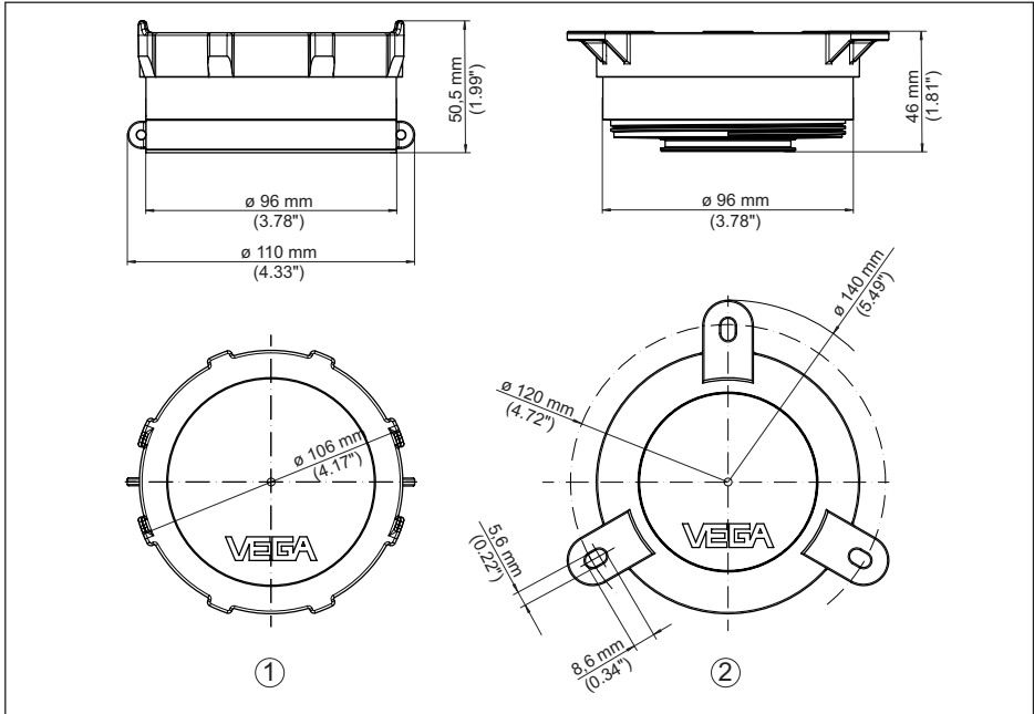
Fig. 18: Dimensions VEGAPULS Air 23
